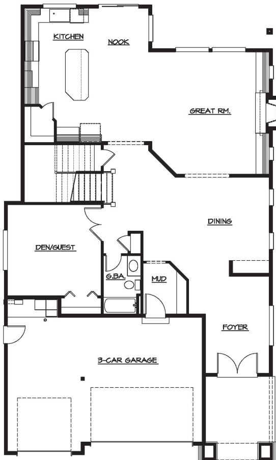
Main Floor
