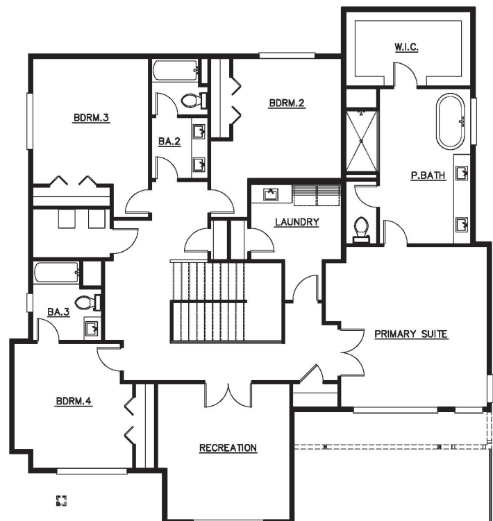
Upper Floor
